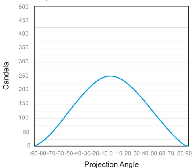
Light distribution of 1 Luxtension
